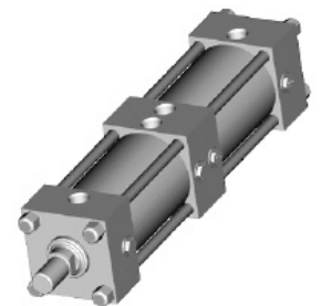
Common Head
