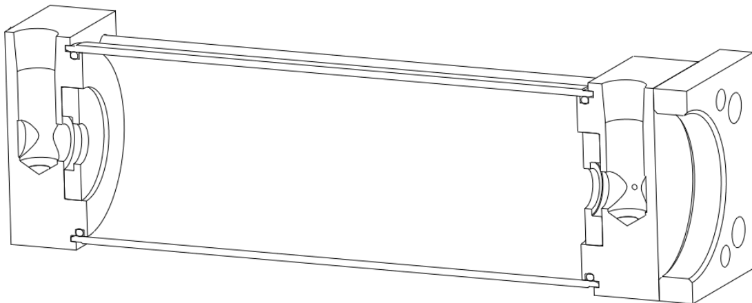
Oil/Air Tank 3.25" bore x 8" Stroke Steel Barrel and heads Custom Mounting End Plate
