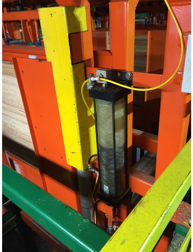
Oil/Air Tank 4" bore x 20" Stroke Clear composite barrel with aluminum heads
